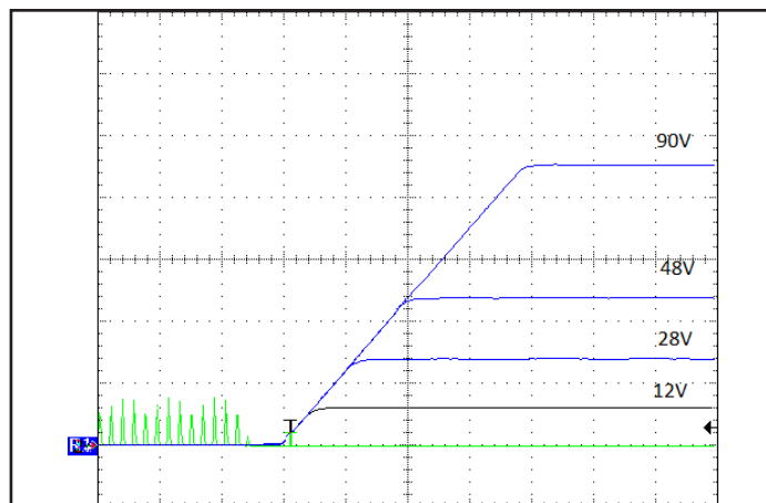
Figure 8: Turn-on transient at 48V input; zero load (10ms/div). Top Traces: Vout (20V/div). Bottom Trace: ON/OFF input (5V/div)
