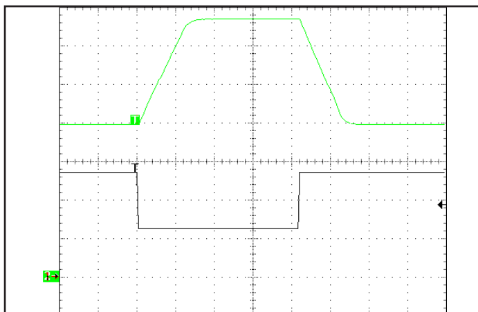
Figure 10: Output Voltage vs. Vset pin voltage dynamics; 48Vin, 2A out (10mS/div). Bottom trace: Vset pin voltage (500mV/div). Top trace: Output Voltage (10V/div).
