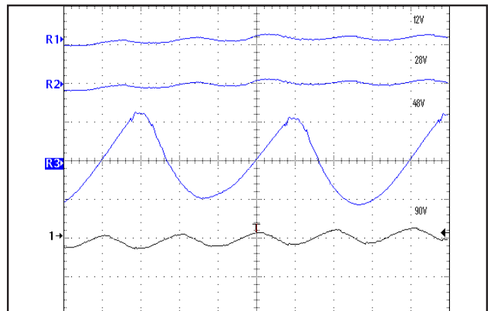
Figure 6: Output Voltage Ripple at 48V input and rated load current (100mV/div). Load capacitance: 100µF electrolytic cap. Bandwidth: 20MHz, (2uS/div). See Figure 4.
