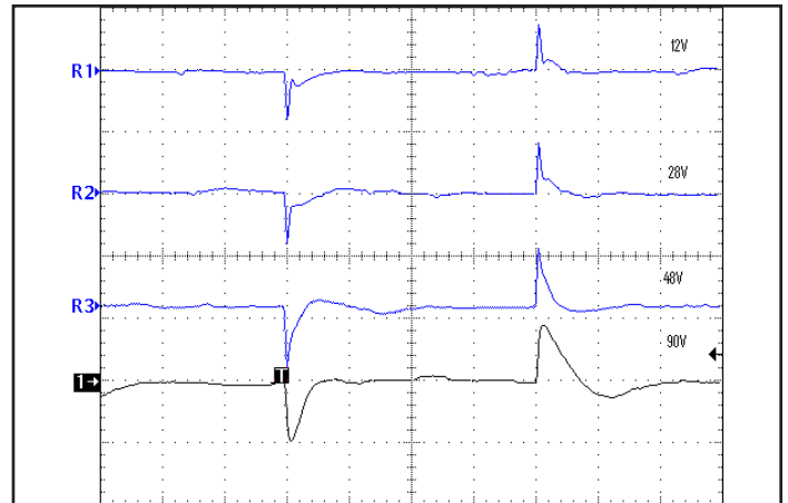
Figure 14: Output voltage response for 48V input; 12V, 28V, 48V, 90V output to step change in load current (50%-75%-50% of I_{out\ max} ; di/dt=0.1A/\mu S ). Load cap: 100uF electrolytic cap, V_{out} (1V/div); (1ms/div)
